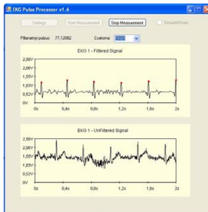
Figure 11 ECG measurements during sudden driving movements
