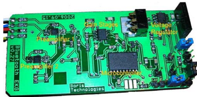
Figure 4 The developed ECG circuit
