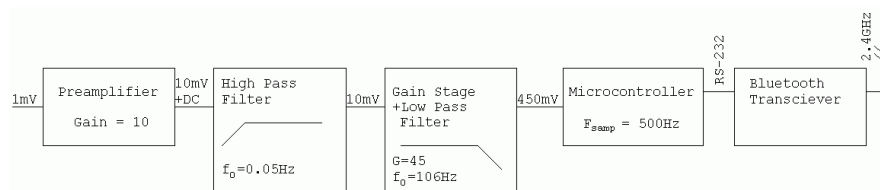
Figure 3 The block diagram of the system
