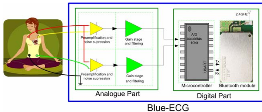
Figure 2 Schematic figure of the developed ECG device
